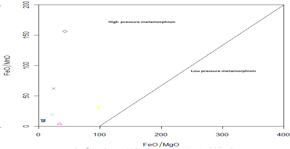
Figure 5: The binary diagram of FeO/MgO versus FeO/MnO in whole rock–comparison of different types of metamorphism (after [30]). Same key as in Figure 4)
