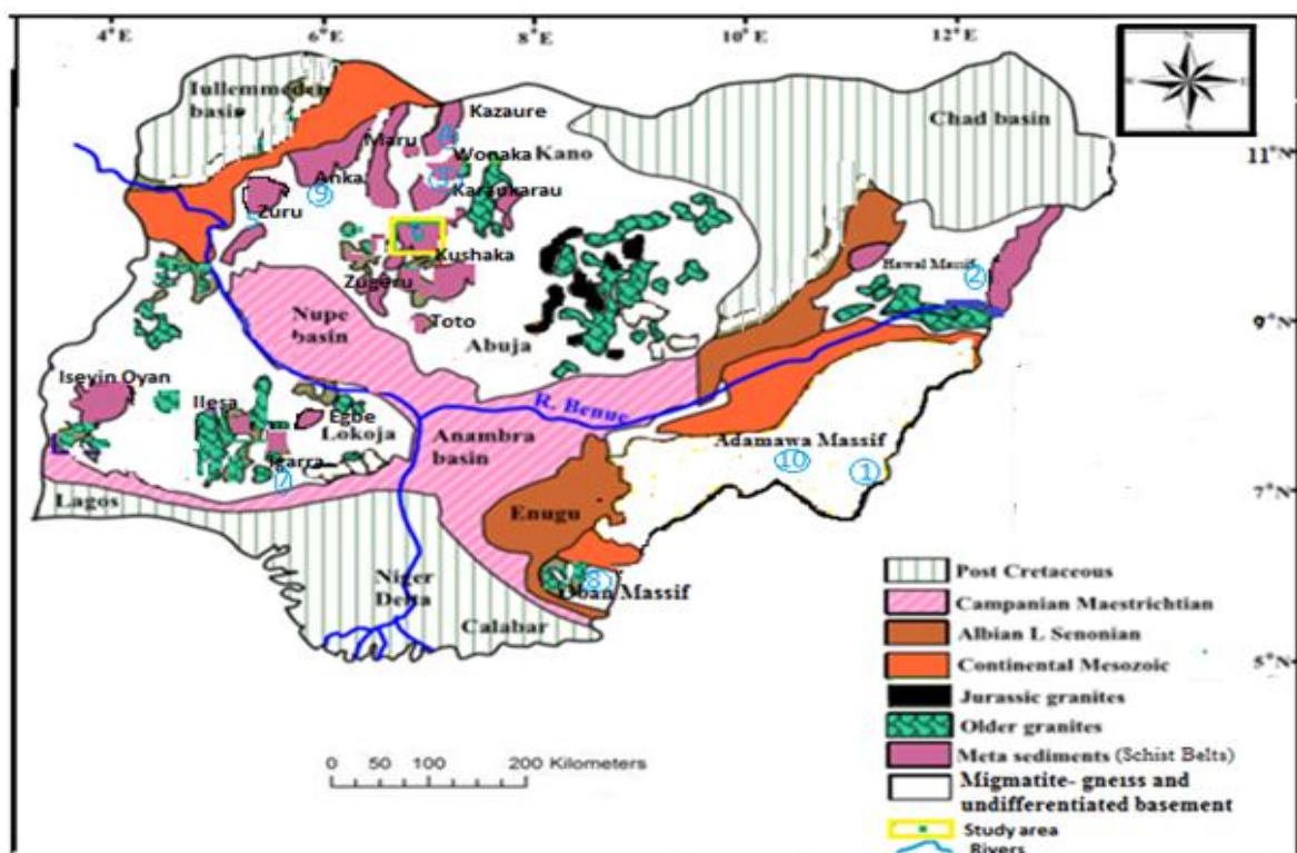
Figure 1: The geological map of Nigeria basement complex and other units of rocks [3].
