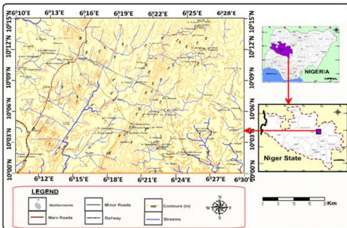
Figure 2: The location and accessibility map of the Madaka and Kwana-Bala area.
