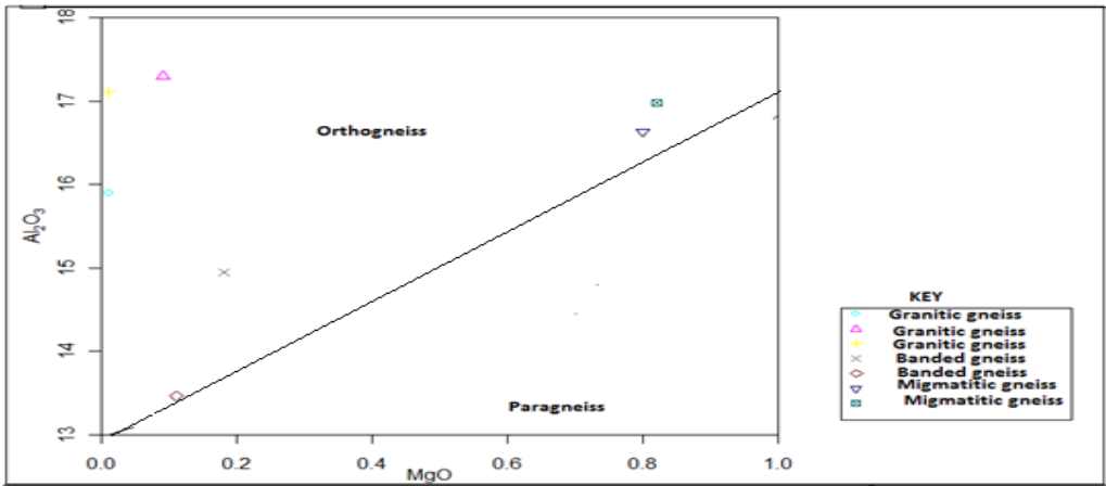
Figure 4: Bivariate Al 2 O 3 versus MgO discrimination diagrams (after [29]) with line that separate paragneiss from orthogneiss for gneisses in the study area.
