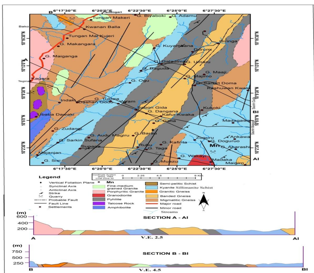
Figure 3: The geological map of the Madaka and Kwana-Bala area
